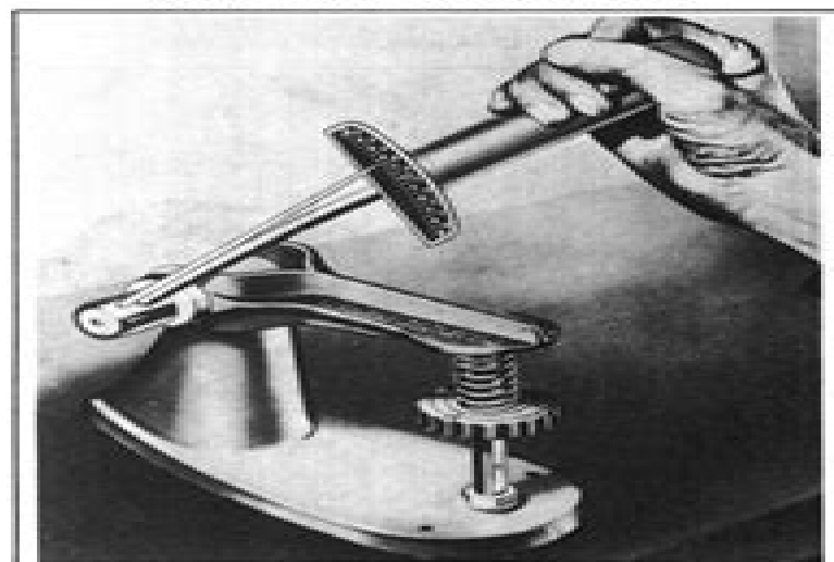
Fig. 6A6-21—Checking Valve Spring Tension
