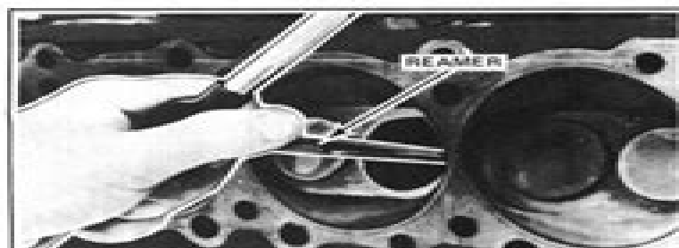
Fig. 6A6-20—Reaming Valve Guide Bore
