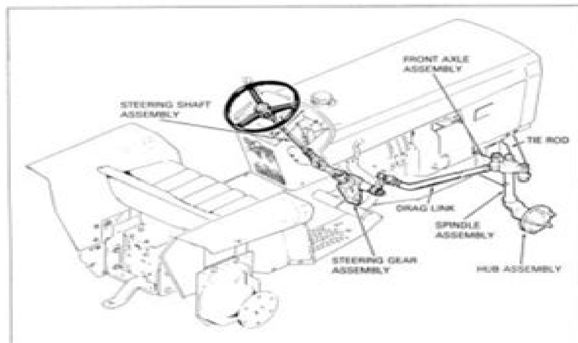
Figure 45. Steering and Front Axle Assemblies
