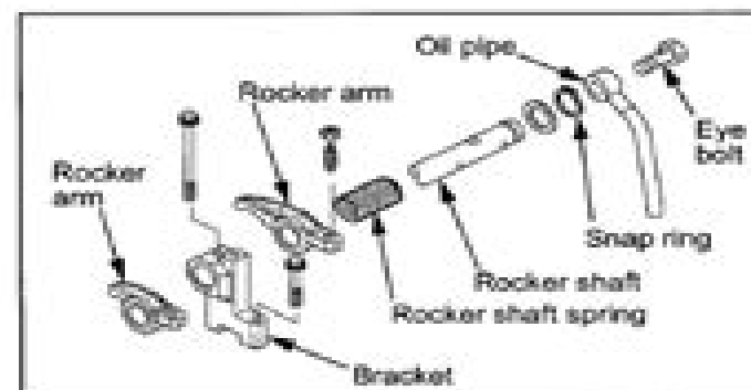
Disassembling rocker shaft assembly
