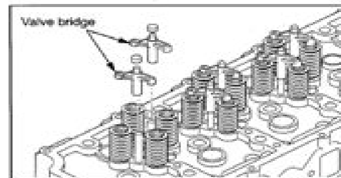
Removing valve bridge
