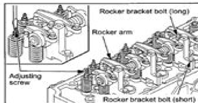
Removing rocker shaft assembly
