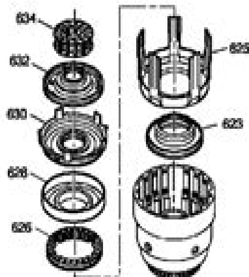
Fig. 147. Input Clutch Assembly Courtesy of GENERAL MOTORS CORP.
