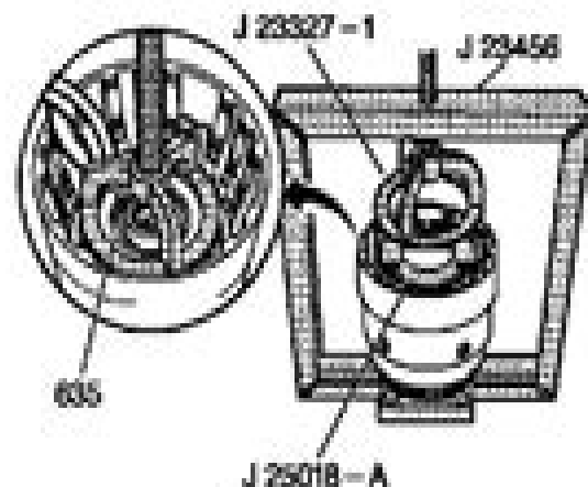
Fig. 146. Installing J 23327-1 & J 23456 Courtesy of GENERAL MOTORS CORP.
