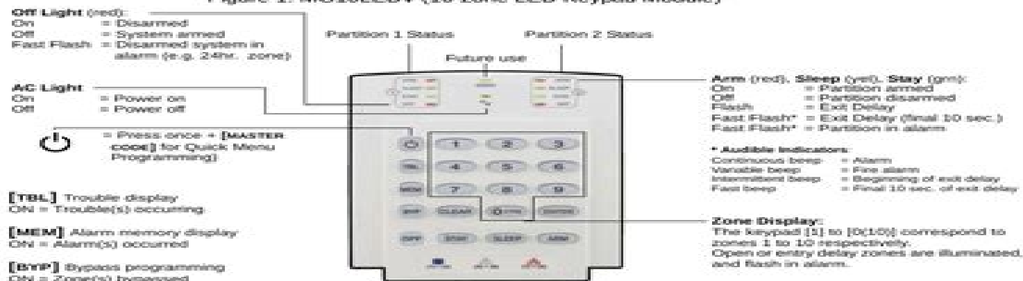
Figure 1: MG10LEDV (10-zone LED Keypad Module)
