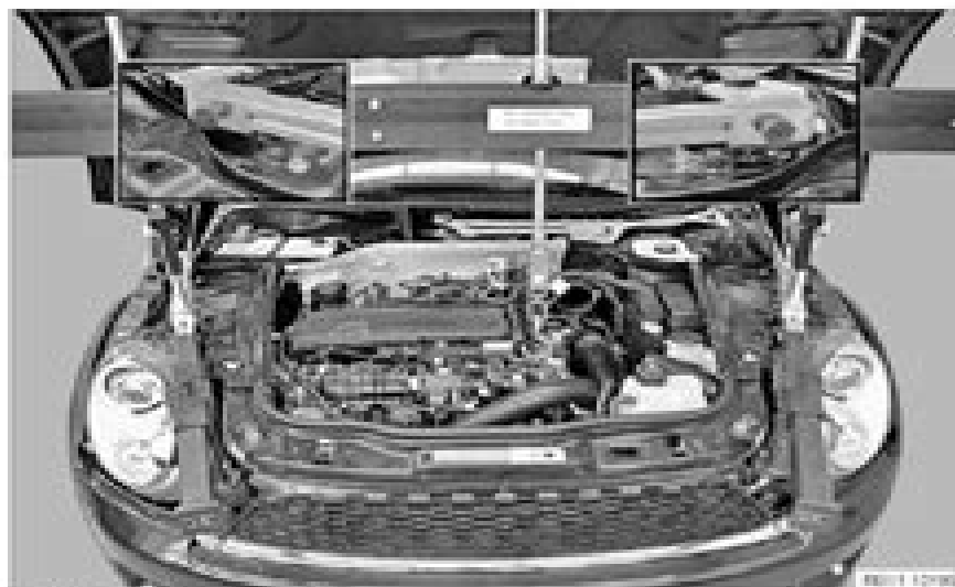
Fig. 12: Positioning Special Tools Courtesy of BMW OF NORTH AMERICA, INC.
