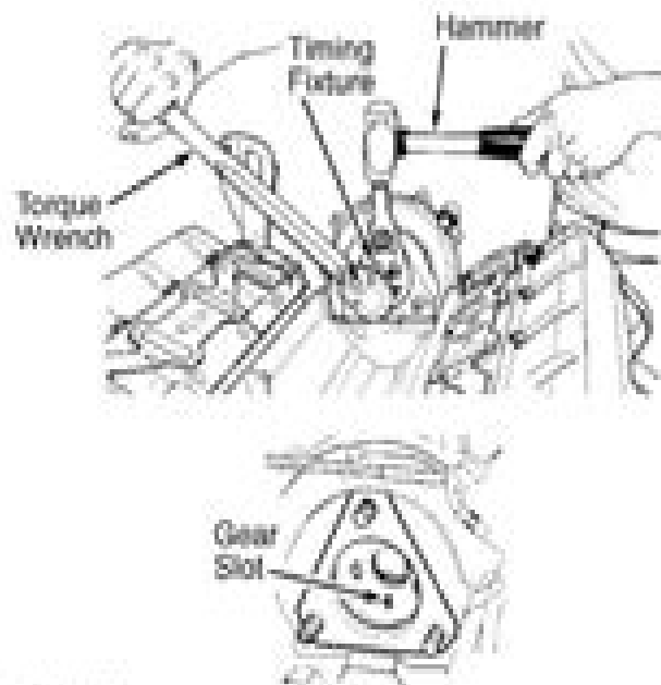
Fig. 1: Marking TDC On Front Cover Courtesy of GENERAL MOTORS CORP.
