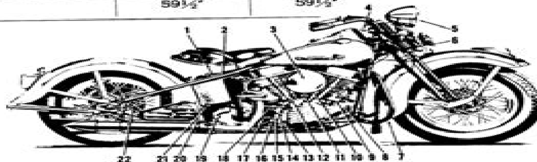
Figure 2 - Right Side View of OHV Model
